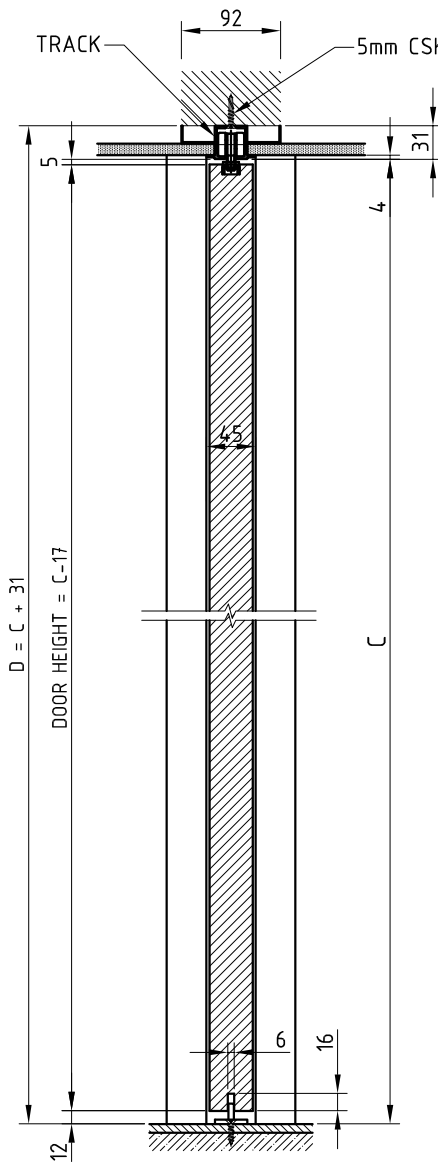
SECTION A - A
